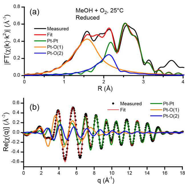
Figure 6. (a) Fourier-transformed ( k = 2.5\text{--}15.5 \text{ \AA}^{-1} ) EXAFS spectrum of the initially reduced catalyst measured at 25 °C in MeOH + \text{O}_2 . The fitted spectrum as well as the magnitudes of the three contributing scattering components corresponding to metallic Pt, a Pt–O(1) bond at \sim 2.0 \text{ \AA} , and Pt–O(2) at \sim 2.5 \text{ \AA} are also shown. (b) Inverse-Fourier-transformed ( R = 1.2\text{--}3.2 \text{ \AA} ) EXAFS spectrum corresponding to that in part a.
