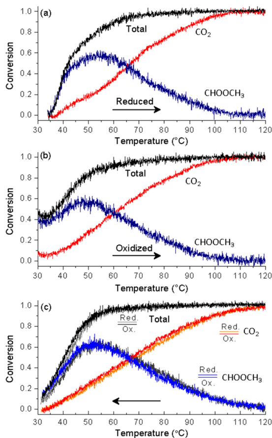
Figure 3. Reactivity of the diluted Pt/ \gamma -Al 2 O 3 catalyst for methanol oxidation. Reactivity following (a) reductive and (b) oxidative pretreatments, measured with increasing temperature. (c) Reactivity following reductive and oxidative pretreatments, measured with decreasing temperature following the measurements shown in a and b.
