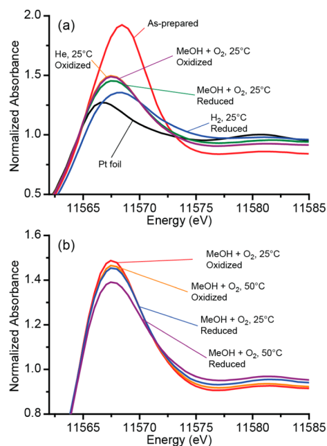
Figure 4. Pt-L 3 XANES spectra of a Pt/ \gamma -Al 2 O 3 catalyst acquired following oxidative and reductive pretreatments and under methanol oxidation conditions after these pretreatments. (a) Comparison of spectra acquired under reaction conditions at room temperature beginning in the reduced state (treated in H 2 at 240 °C) and an oxidized state (treated in O 2 at 240 °C), respectively. XANES spectra acquired of the as-prepared (oxidized) catalyst and of a bulk Pt foil are shown for reference. (b) Comparison of spectra acquired under reaction conditions at different temperatures.
