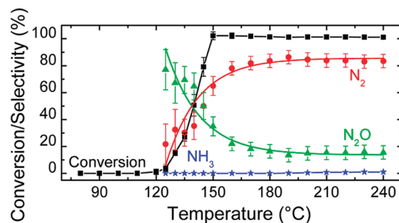
Figure 3. Conversion and selectivity data as a function of temperature for the steady state H 2 -SCR NO reduction over micellar Pd NPs supported on ZrO 2 .
