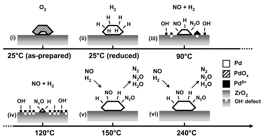
Figure 8. Schematic representation of the structure and chemical state of our Pd nanocatalysts at various stages of the H 2 -SCR NO reduction.
