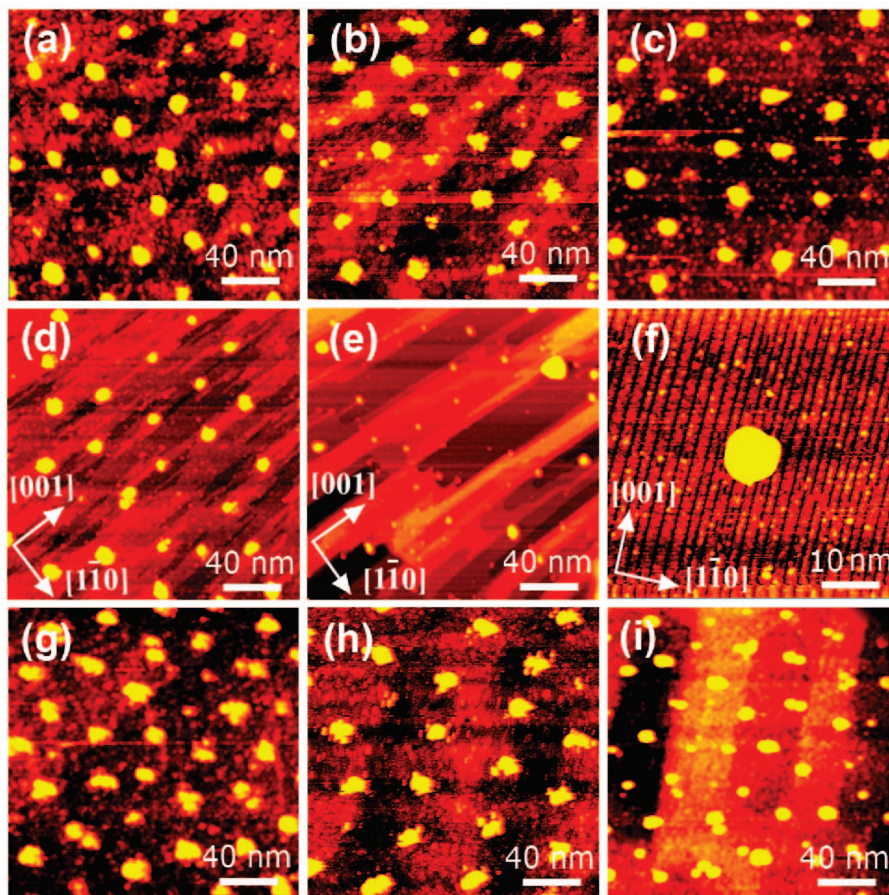
Figure 3. STM images of bimetallic \text{Au}_{0.5}\text{Fe}_{0.5} (a–f), pure Au (g,h) and pure Fe (i) nanoparticles supported on \text{TiO}_2(110) and measured at 15 °C after an in situ \text{O}_2 plasma treatment and subsequent annealing at: (a,g) 300 °C, (b,i) 700 °C, (c) 800 °C, (d,h) 900 °C, and (e,f) 1000 °C. With the exception of image (f) ( 50 \times 50 \text{ nm}^2 ), the rest of the images correspond to a scan region of ( 200 \times 200 \text{ nm}^2 ).
