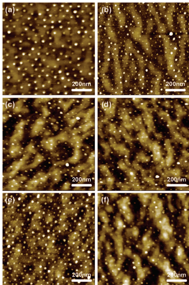
Figure 1. AFM images of (a) Au, (b) Fe, (c–f) Au 0.5 Fe 0.5 nanoparticles synthesized by inverse micelle encapsulation in PS(81000)-P2VP(142000) and supported on TiO 2 (110). The images were taken in air after polymer removal in UHV by an O 2 -plasma treatment (a–c) and subsequent annealing of the Au 0.5 Fe 0.5 NPs at 500 °C (d), 700 °C (e), and 900 °C (f).
