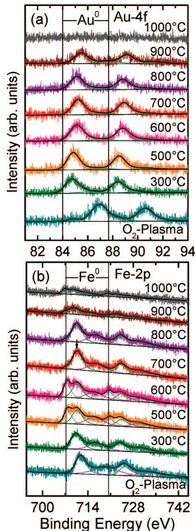
Figure 8. XPS spectra of (a) the Au-4f and (b) Fe-2p core level regions of Au 0.5 Fe 0.5 nanoparticles supported on TiO 2 (110). The spectra were acquired after O 2 plasma treatment and after subsequent in situ annealing from 300–700 °C for 20 min and from 800–1000 °C for 10 min. The arrow in (b) at a BE of 710.7 eV indicates the position of the XPS peak corresponding to Fe in an Fe–Au alloy after annealing at 700 °C. Accidentally, a similar BE is observed for oxidized Fe species and/or FeTiO 3+δ compounds at the Fe/TiO 2 interface in pure Fe clusters. The corresponding spectral least-squares fits for the different Au and Fe species are also shown, (solid lines).
