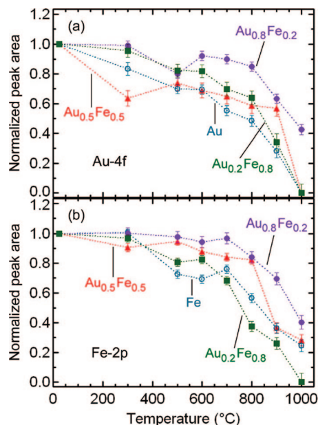
Figure 13. Evolution of the (a) Au-4f and (b) Fe-2p XPS normalized spectral areas (integrated intensities) of Au (○), Fe (○), and Au x Fe 1-x [ x = 0.8 (●), 0.5 (▲), 0.2 (■)] nanoparticles supported on TiO 2 (110) with annealing temperature. These data were extracted from the XPS spectra displayed in Figures 6, 7, 8, and 10. The spectral areas were calculated from the least-squares fits of the XPS peaks using the CasaXPS software considering a linear background and a Gaussian–Lorentzian line-shape. The data are normalized using the respective XPS spectral area measured directly after O 2 –plasma treatment as reference.
