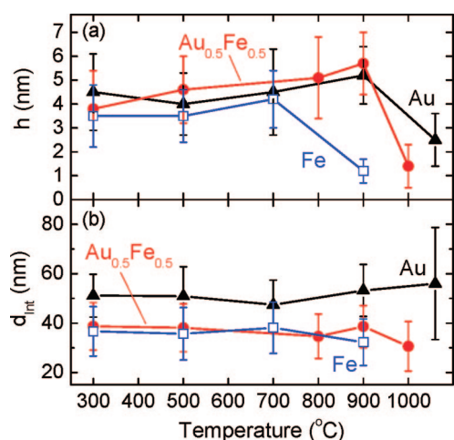
Figure 5. Evolution of the (a) average height ( h ) and (b) interparticle distance ( d_{\text{int}} ) of Au 0.5 Fe 0.5 (●), Au (▲) and Fe (□) nanoparticles with annealing temperature. The error bars given correspond to the standard deviation calculated from the distribution of particle heights and interparticle distances: shown in Figure 4.
