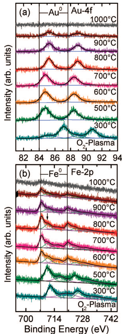
Figure 6. XPS spectra of (a) the Au-4f and (b) Fe-2p core level regions of pure Au (a) and pure Fe (b) nanoparticles supported on TiO 2 (110). The spectra were acquired after O 2 -plasma treatment and after subsequent in situ annealing from 300 to 700 °C for 20 min and from 800 to 1000 °C for 10 min. The reference straight solid lines indicate the binding energies of bulk Au and Fe. The arrow in (b) at a BE of 710.5 eV indicates the presence of oxidized Fe species (Fe 2+ /Fe 3+ ) and/or an FeTiO 3+δ compound at the Fe/TiO 2 interface after annealing at 700 °C. The corresponding spectral least-squares fits for the different Au and Fe species are also shown, (solid lines).
