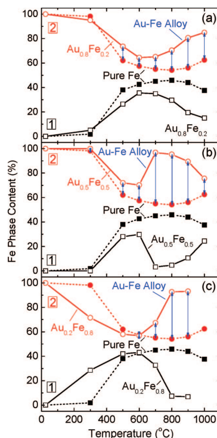
Figure 12. Evolution of the relative content (spectral area) of the two different Fe phases (component 1 and component 2) obtained from the fits of Fe-2p XPS spectra acquired after sample annealing in UHV from RT to 1000 °C. The data shown correspond to the following samples: (a) \text{Au}_{0.8}\text{Fe}_{0.2} , (b) \text{Au}_{0.5}\text{Fe}_{0.5} , and (c) \text{Au}_{0.2}\text{Fe}_{0.8} NPs, ( \square and \circ connected by solid lines). For comparison, the phase content of the pure Fe NPs is also plotted ( \blacksquare and \bullet connected by dashed lines). The component labeled as 1 (squares) corresponds to the low BE feature (Fe-2p 3/2 at 706.9–707.7 eV) assigned to metallic Fe, while component 2 corresponds to the high BE feature (Fe-2p 3/2 at 709.8–712.2 eV and satellites at \sim 720 eV) attributed to Fe–oxides + \text{FeTiO}_{3+\delta} compounds + Au–Fe alloy. These data were extracted from the XPS spectra displayed in Figures 6, 7, 8, and 10. The vertical arrows indicate the increase in the phase content of component 2 in the \text{Au}_x\text{Fe}_{1-x} nanoparticles relative to the phase content of component 2 in the pure Fe NPs. This increase is attributed to the formation of an Au–Fe alloy.
