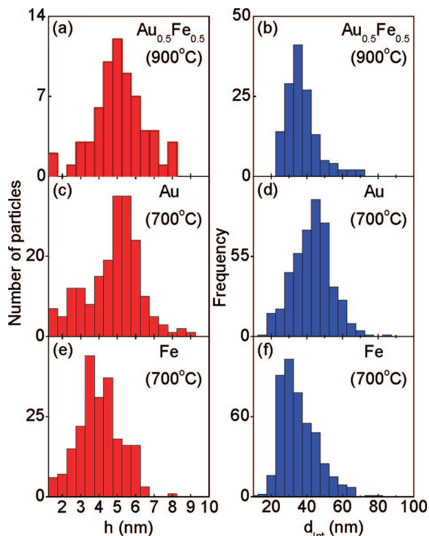
Figure 4. Representative histograms of the size and interparticle distance of Au 0.5 Fe 0.5 (a,b), Au (c,d), and Fe (e,f) NPs synthesized by inverse micelle encapsulation with PS(81000)-PVP(14200) and deposited on TiO 2 (110). The data were extracted from a series of STM images acquired after polymer removal by an in situ atomic oxygen treatment and subsequent annealing in UHV at 900 °C (a,b) and 700 °C (c–f).
