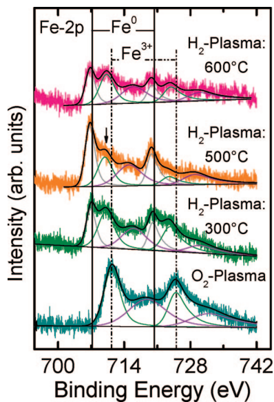
Figure 9. XPS spectra of the Fe-2p core level region from a sample containing \text{Au}_{0.5}\text{Fe}_{0.5} NPs deposited on \text{TiO}_2(110) . The sample was first exposed to an \text{O}_2 -plasma treatment in UHV for 80 min and subsequently to \text{H}_2 -plasma treatments (60 min each) at 300, 500, and 600 °C. At 500 °C, the arrow at a BE of 710 eV indicates the presence of an Au-Fe alloy. The corresponding spectral least-squares fits for the different Fe species are also shown.
