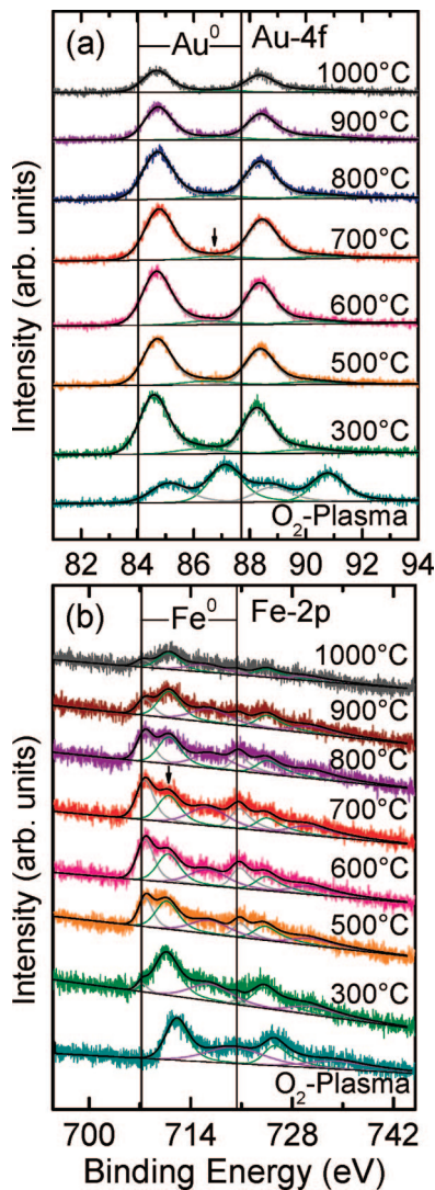
Figure 7. XPS spectra of (a) the Au-4f and (b) Fe-2p core level regions of Au 0.8 Fe 0.2 nanoparticles supported on TiO 2 (110). The spectra were acquired after O 2 plasma treatment and after subsequent in situ annealing from 300–700 °C for 20 min and from 800–1000 °C for 10 min. The arrow in (b) at a BE of 710.5 eV indicates the position of a XPS peak corresponding to the partial formation of an Fe–Au alloy after annealing at 700 °C. Coincidentally, a similar BE is observed for oxidized Fe species and/or FeTiO 3+δ compounds at the Fe/TiO 2 interface in pure Fe clusters. The corresponding spectral least-squares fits for the different Au and Fe species are also shown, (solid lines).
