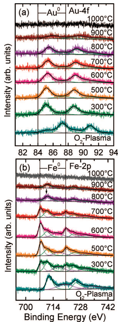
Figure 10. XPS spectra of (a) the Au-4f and (b) Fe-2p core level regions of \text{Au}_{0.2}\text{Fe}_{0.8} nanoparticles supported on \text{TiO}_2(110) . The spectra were acquired after \text{O}_2 plasma treatment and after subsequent in situ annealing from 300 to 700 °C for 20 min and from 800 to 1000 °C for 10 min. The arrow in (b) at a BE of 710.5 eV indicates the position of the XPS peak corresponding to Fe in a Fe-Au alloy after annealing at 800 °C. Coincidentally, a similar BE is observed for oxidized Fe species and/or \text{FeTiO}_{3+\delta} compounds at the Fe/ \text{TiO}_2 interface in pure Fe clusters. The corresponding spectral least-squares fits for the different Au and Fe species are also shown.
