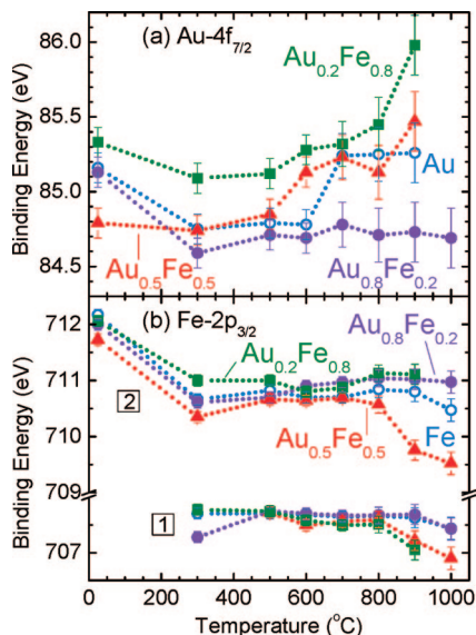
Figure 11. Evolution of the (a) Au-4f 7/2 and (b) Fe-2p 3/2 binding energies of Au (○), Fe (○), and Au x Fe 1-x [ x = 0.8 (●), 0.5 (▲), 0.2 (■)] nanoparticles supported on TiO 2 (110) with annealing temperature. In (b), the component labeled as 1 corresponds to metallic Fe (Fe-2p 3/2 BE of 706.9–707.7 eV), while component 2 (Fe-2p 3/2 BE of 709.8–712.2 eV) includes Fe–oxides + FeTiO 3+δ + Au–Fe alloy compounds, which cannot be distinguished based on the BE. These data were extracted from the XPS spectra displayed in Figures 6, 7, 8, and 10.
