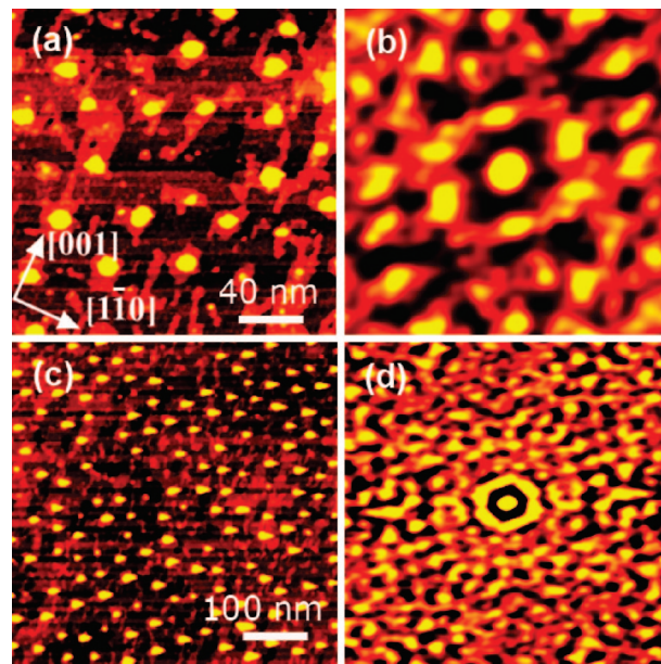
Figure 2. STM (a,c) and corresponding spatial autocorrelation images (b,d) of Au 0.5 Fe 0.5 nanoparticles synthesized by inverse micelle encapsulation and supported on TiO 2 (110). The images were taken after sample annealing in UHV at 900 °C for 20 min.
