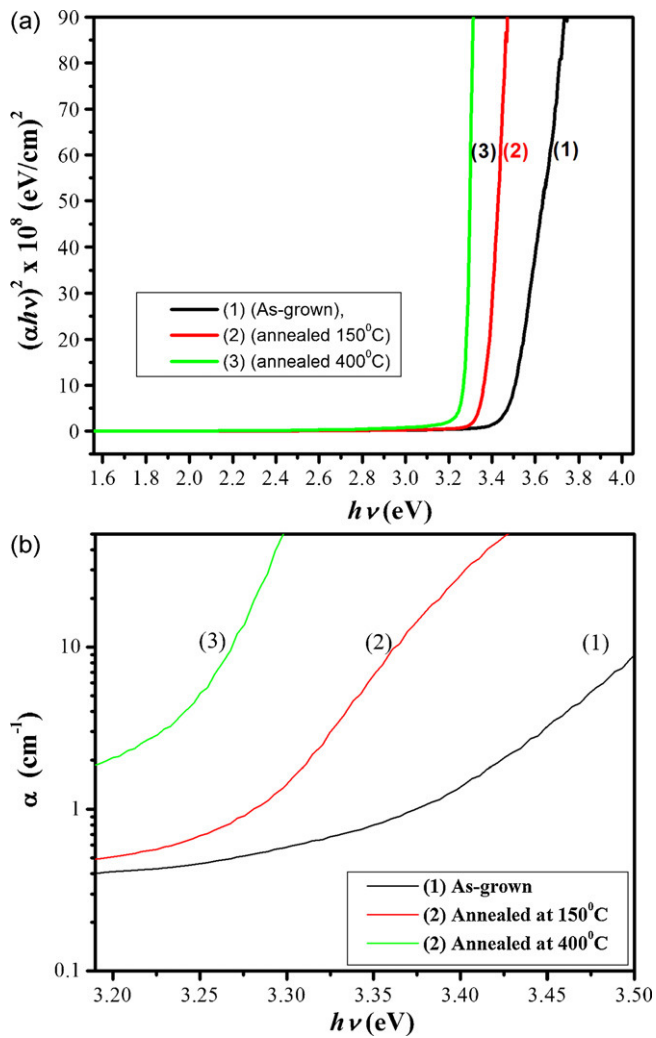
Fig. 12. (a) Plot of (\alpha hv)^2 vs. photon energy for ZnO films as-grown and annealed at 150 and 400 °C, respectively. (b) Plot of absorption coefficient near the UV edge vs. photon energy ( h\nu ) for ECD ZnO thin films.
