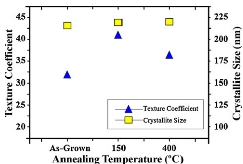
Fig. 3. Variation of the texture coefficient TC_{(002)} and mean crystallite size with thermal annealing temperature of ECD ZnO thin films. Mean crystallite size: as-grown, 2180 Å; 150^\circ\text{C} , 2189 Å; and 400^\circ\text{C} , 2189 Å.
